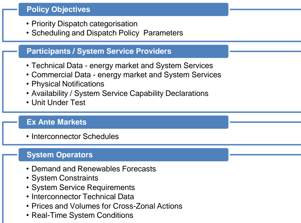
Figure 3: Inputs to the Scheduling and Dispatch Process
