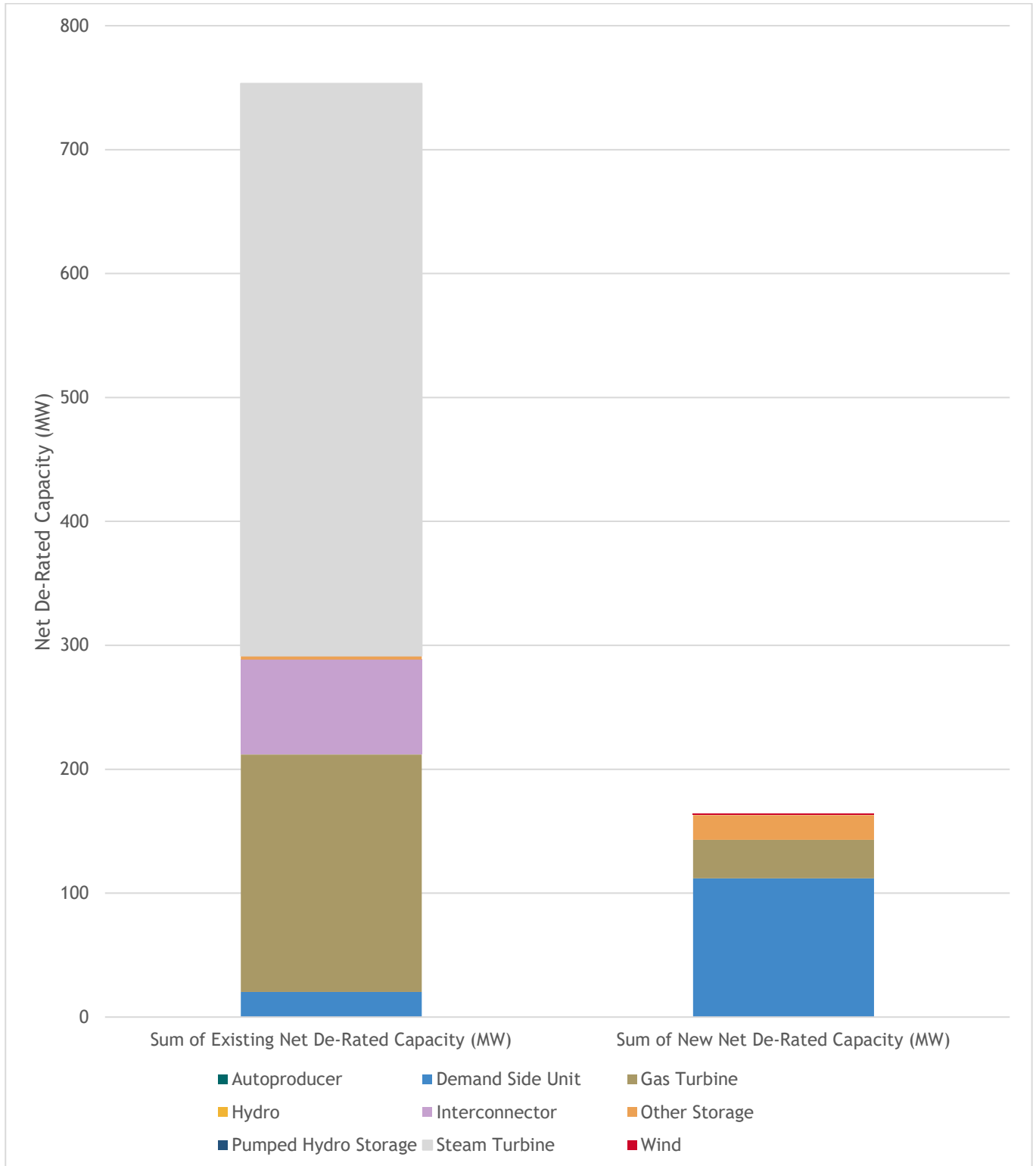
Figure 1 - New and Existing Qualified Capacity by Unit Type / Technology Class
